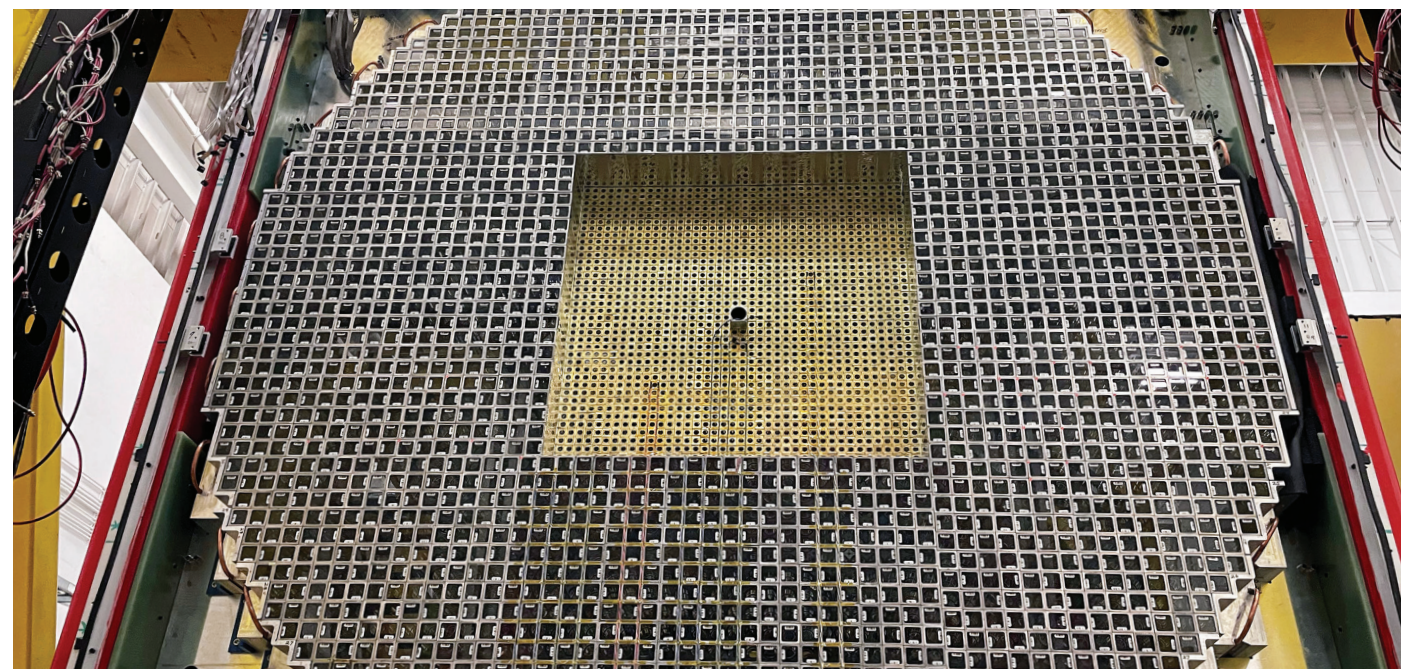
The upgraded forward electromagnetic calorimeter with lead-tungstate crystals in Experimental Hall D at Jefferson Lab.
