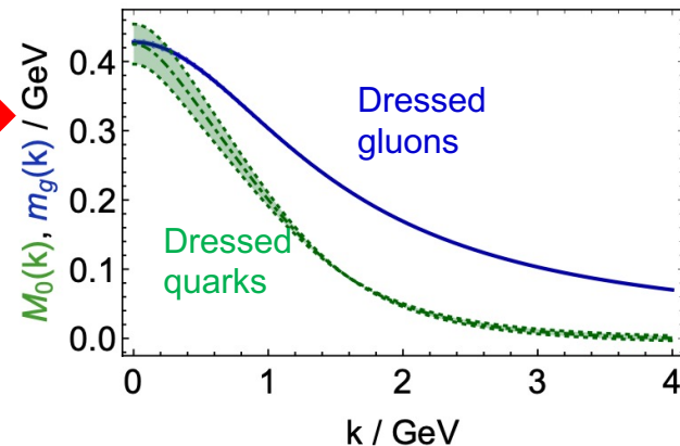
Dressed Quark/Gluon Running Masses
