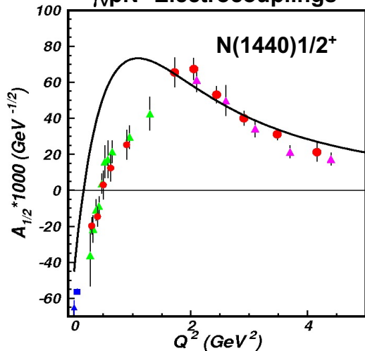
\gamma_p p N^* Electrocouplings
