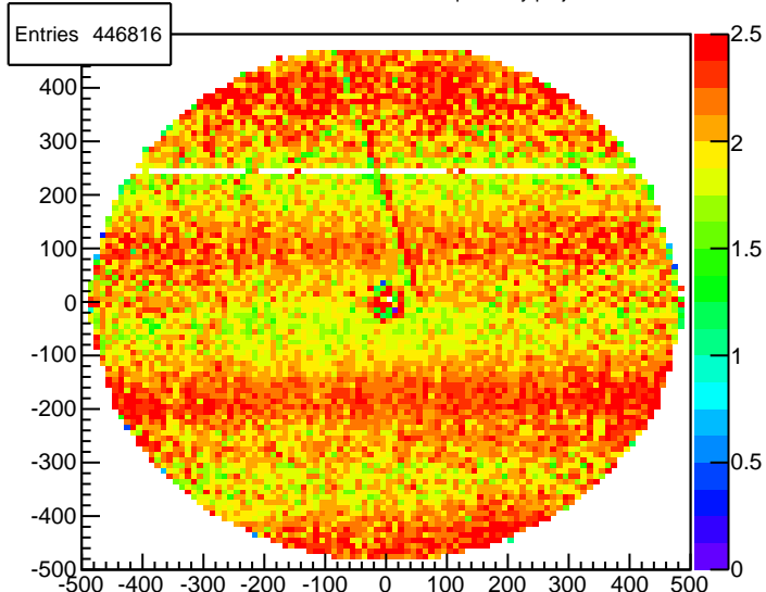
FDC3 Cell4 Cathode x-nominal wire profile xy projection
