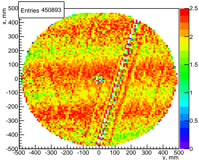
FDC3 Cell5 Cathode x-nominal wire profile xy projection
