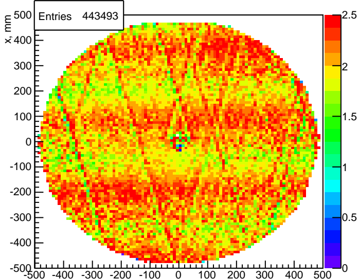
FDC3 Cell1 Cathode x-nominal wire profile xy projection
