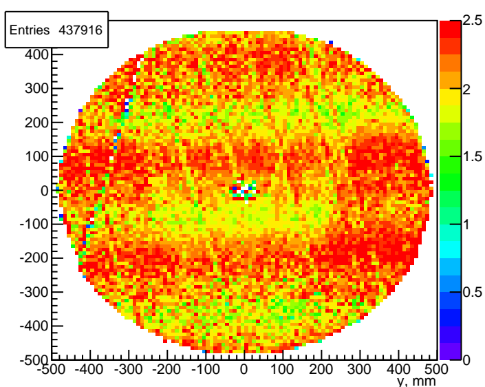
FDC3 Cell6 Cathode x-nominal wire profile xy projection
