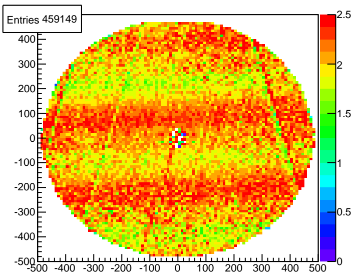
FDC3 Cell2 Cathode x-nominal wire profile xy projection
