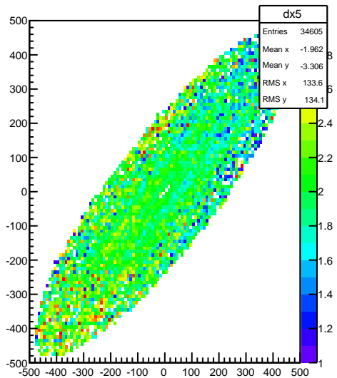
FDC1 Cell6 Cathode x-nominal wire profile xy projection
