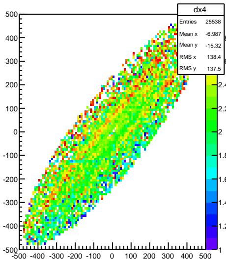
FDC1 Cell5 Cathode x-nominal wire profile xy projection
