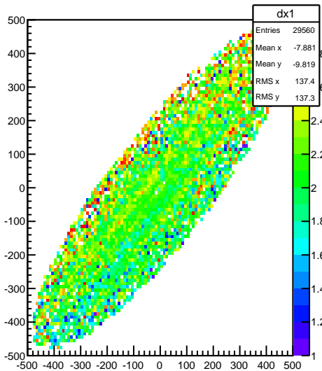
FDC1 Cell2 Cathode x-nominal wire profile xy projection
