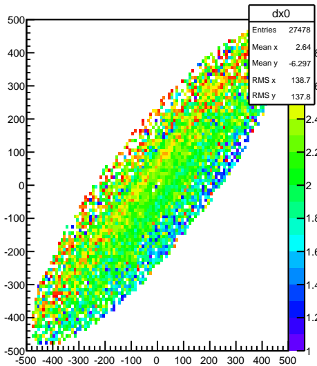
FDC1 Cell1 Cathode x-nominal wire profile xy projection
