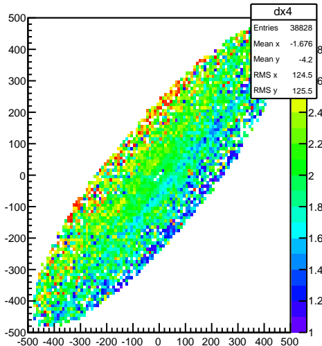
FDC2 Cell5 Cathode x-nominal wire profile xy projection
