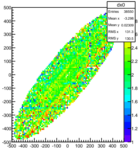
FDC2 Cell1 Cathode x-nominal wire profile xy projection
