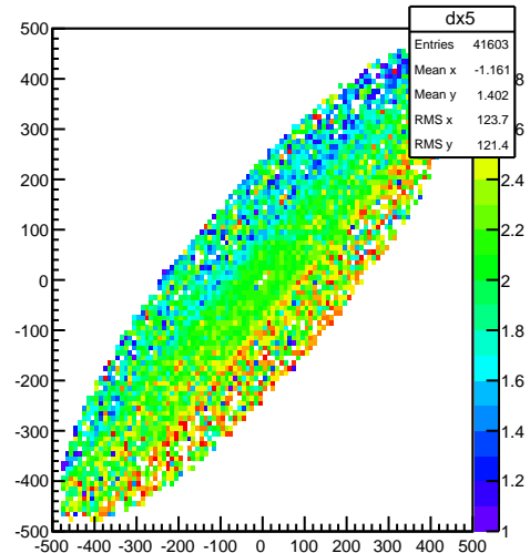
FDC2 Cell6 Cathode x-nominal wire profile xy projection
