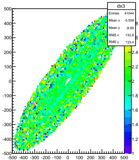
FDC3 Cell4 Cathode x-nominal wire profile xy projection
