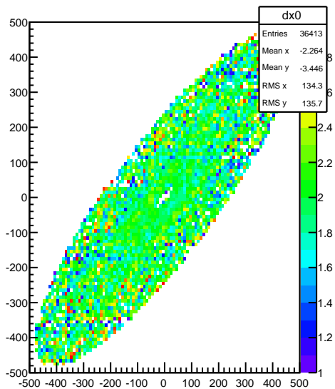
FDC3 Cell1 Cathode x-nominal wire profile xy projection
