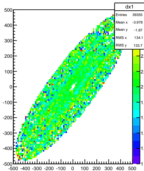
FDC3 Cell2 Cathode x-nominal wire profile xy projection
