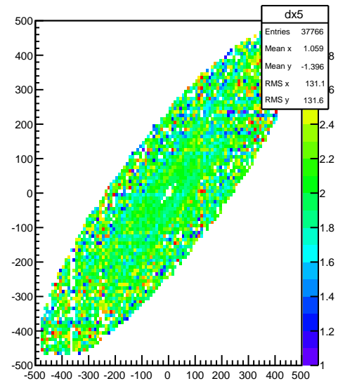
FDC3 Cell6 Cathode x-nominal wire profile xy projection
