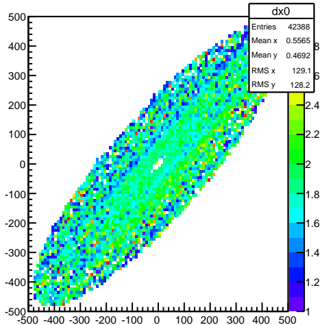
FDC4 Cell1 Cathode x-nominal wire profile xy projection
