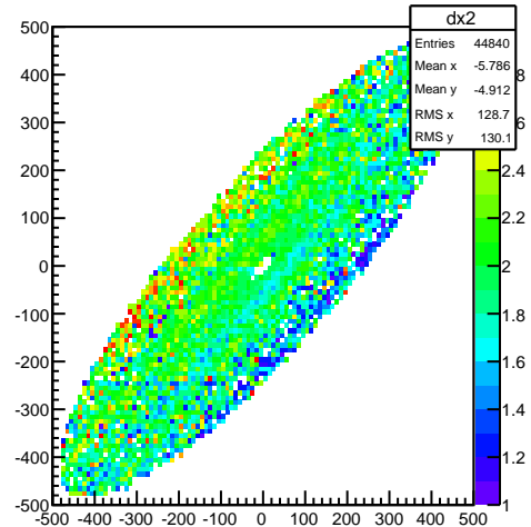
FDC4 Cell3 Cathode x-nominal wire profile xy projection
