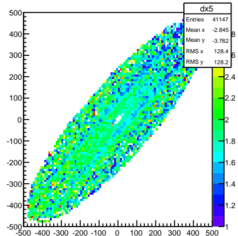
FDC4 Cell6 Cathode x-nominal wire profile xy projection
