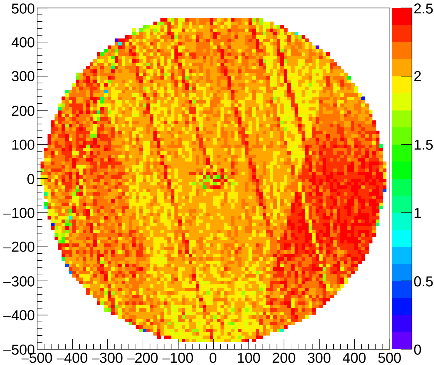
FDC3 Cell6 Cathode x-nominal wire profile xy projection
