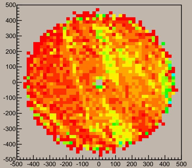
FDC3 Cell6 Normalization for cathode y-reconstr.from track
