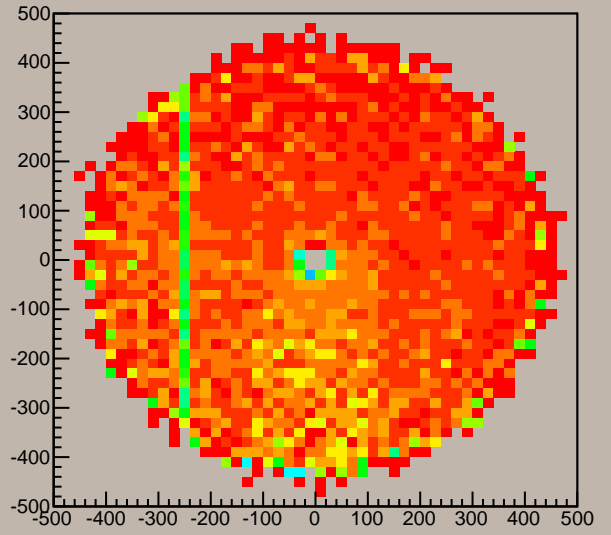
FDC3 Cell4 Normalization for cathode y-reconstr.from track
