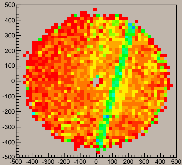
FDC3 Cell5 Normalization for cathode y-reconstr.from track
