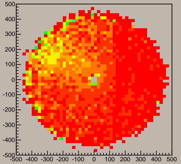
FDC3 Cell2 Normalization for cathode y-reconstr.from track
