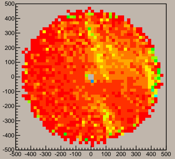
FDC3 Cell6 Normalization for cathode y-reconstr.from track
