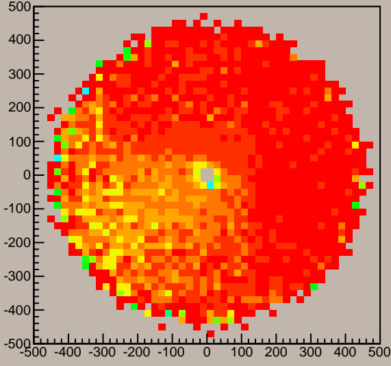
FDC3 Cell3 Normalization for cathode y-reconstr.from track
