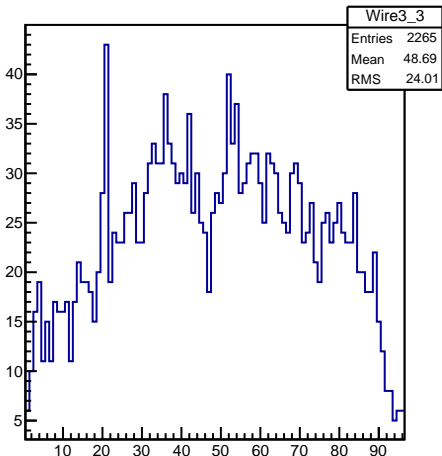
FDC4 Cell4 wire hits
