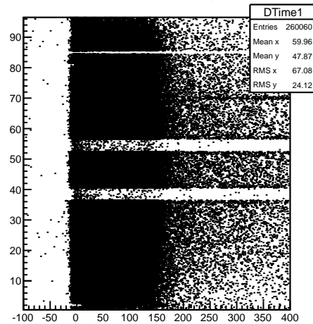
Drift Time vs wire no., cell 1
