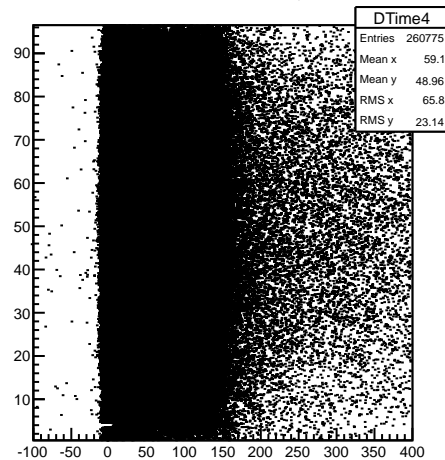
Drift Time vs wire no., cell 4
