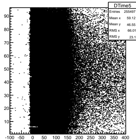
Drift Time vs wire no., cell 5
