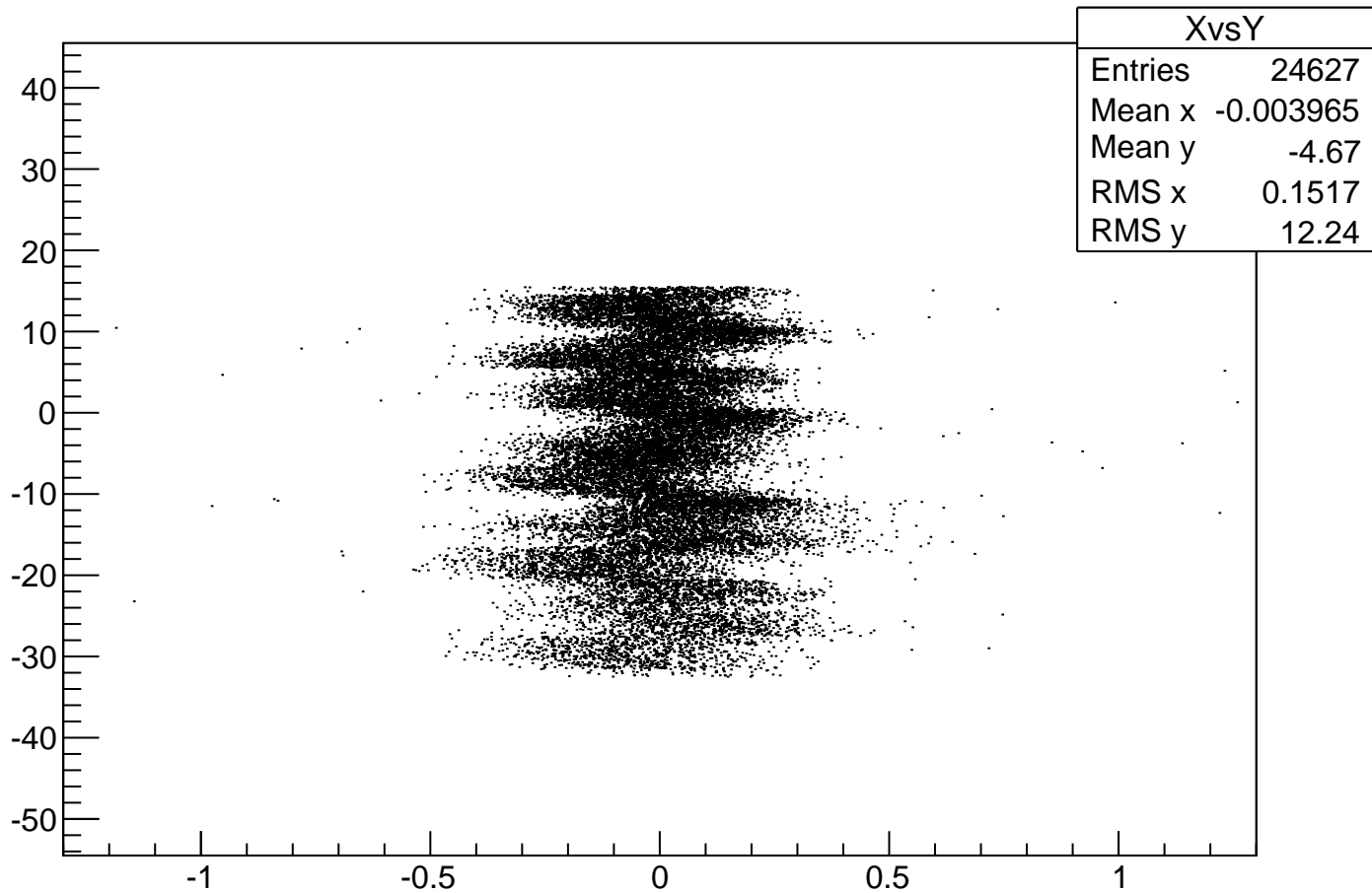
cathode reconstructed X position vs distance along wire
