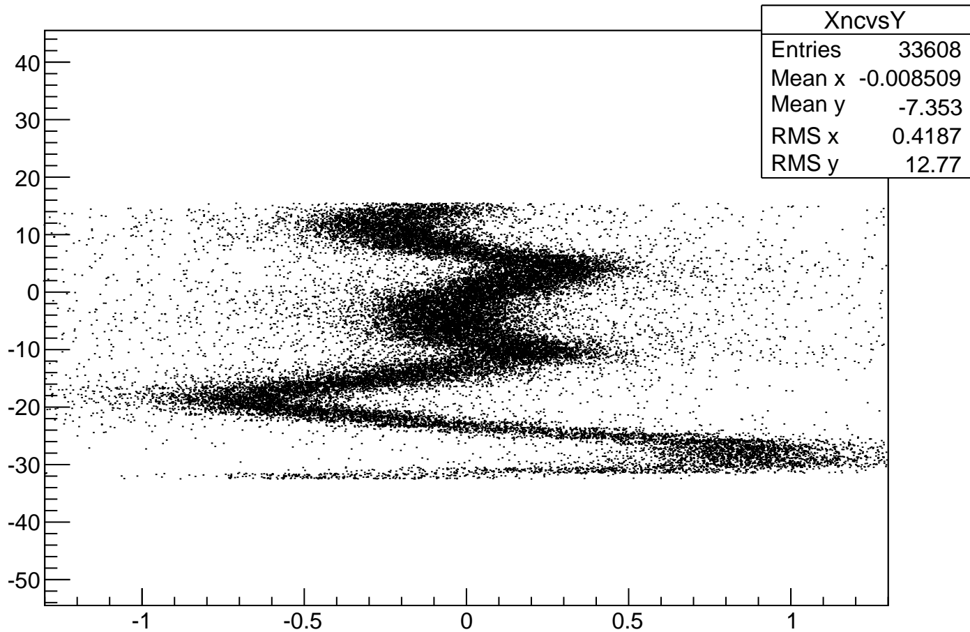
cathode reconstructed X position (not corrected) vs distance along wire
