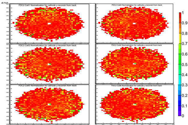
Figure: Package 2 efficiency, x and y in mm
