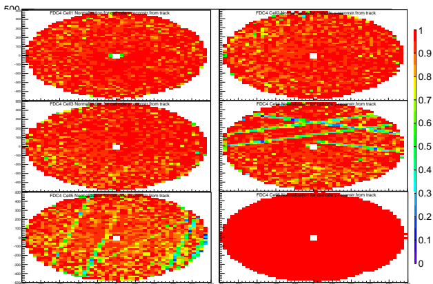
Figure: Package 4 efficiency, x and y in mm
