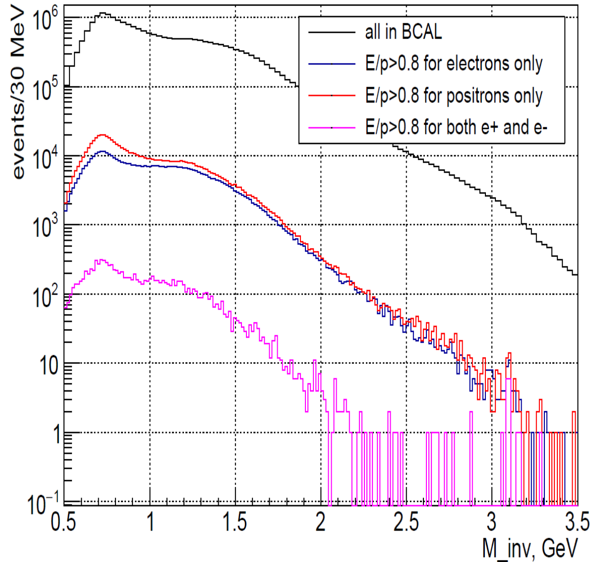
Invariant Mass Spectrum with E/p cuts
