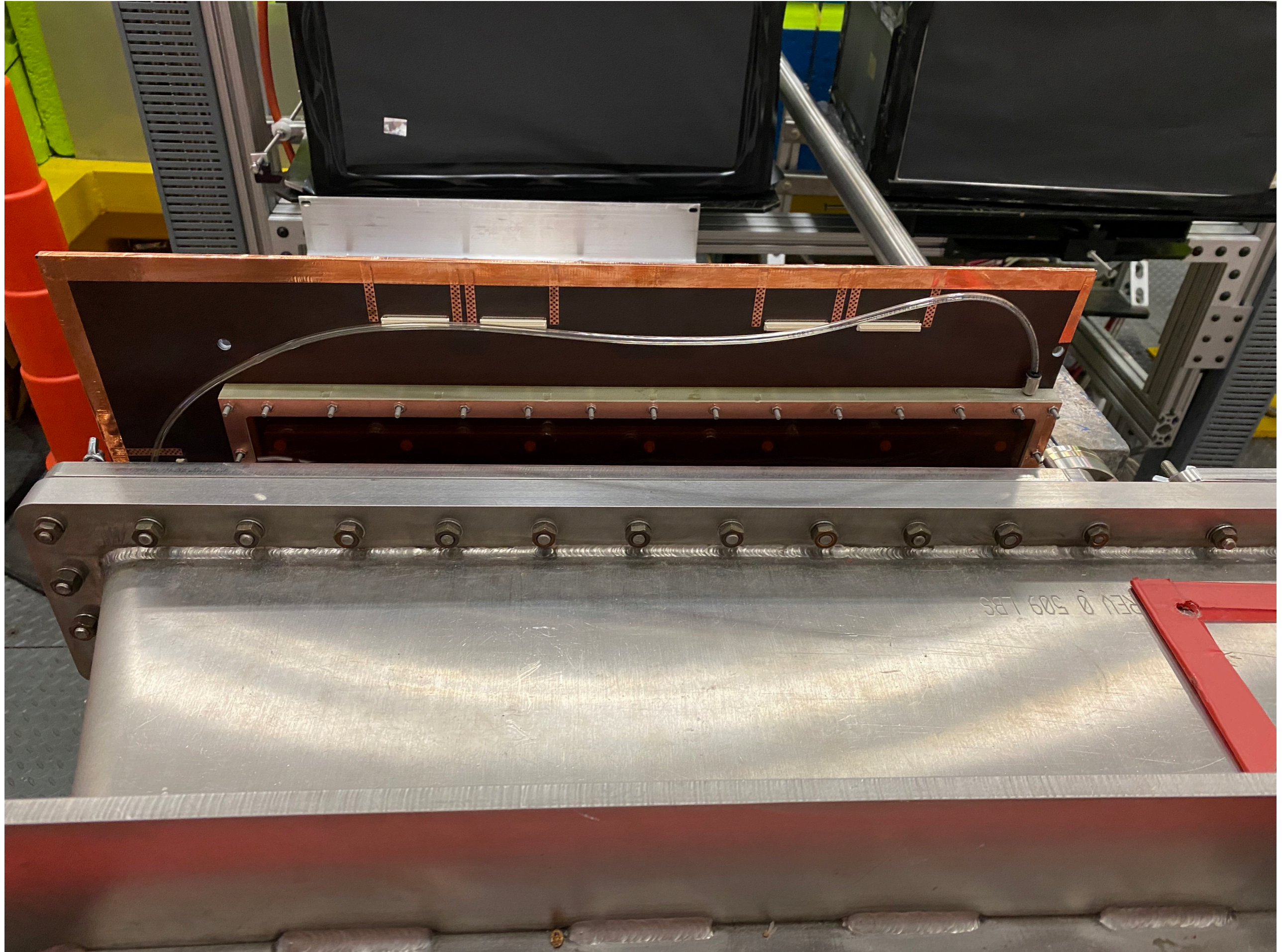
GEM setup at PS
