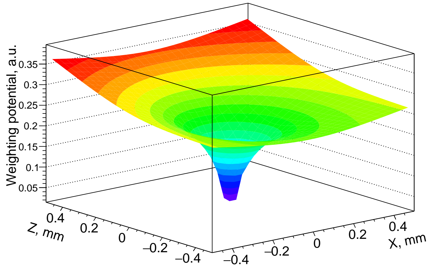
Weighting field for top cathode (positive Z)
