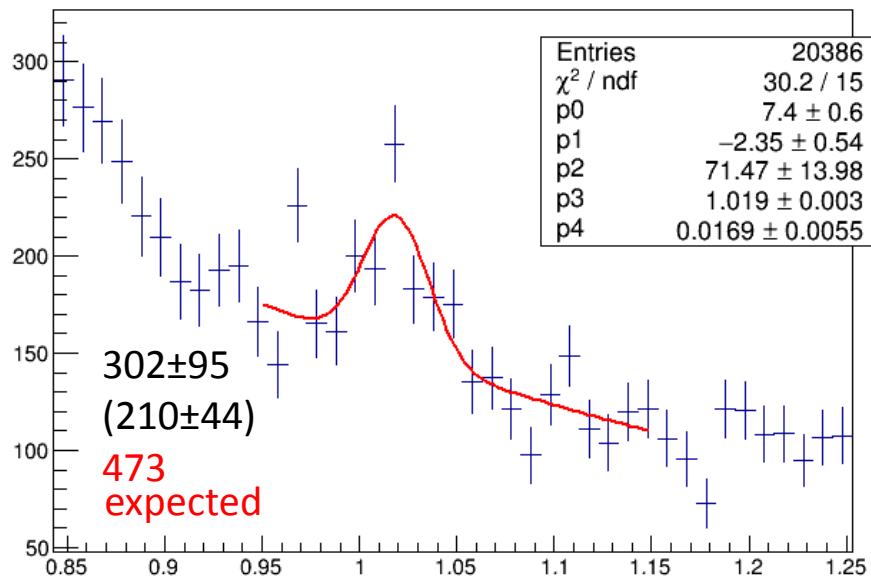
\phi 2017 high 0 < \chi^2 < 5000
