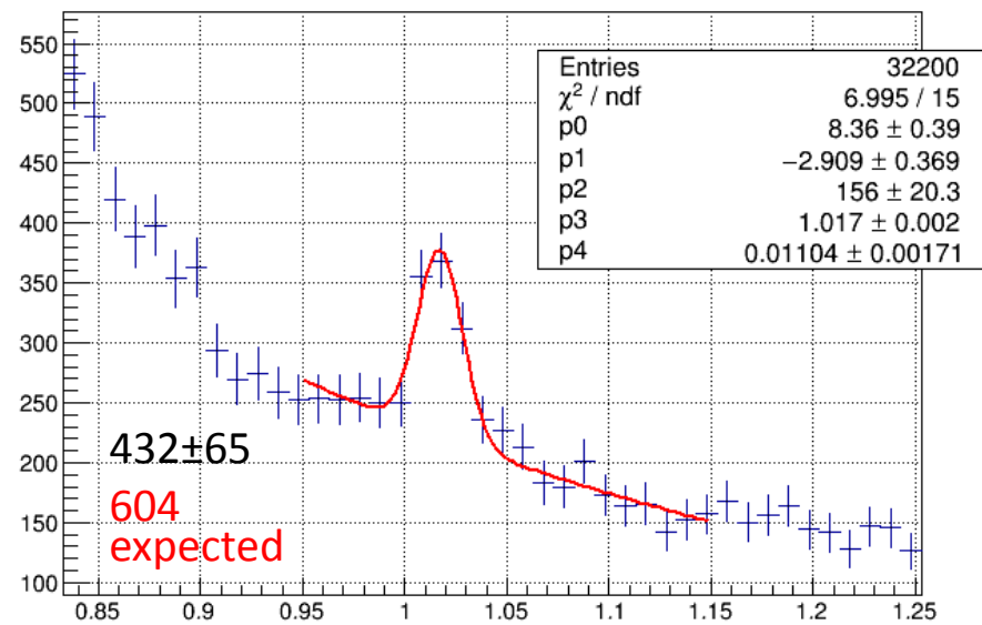
\phi 2017 low 0 < \chi^2 < 5000
