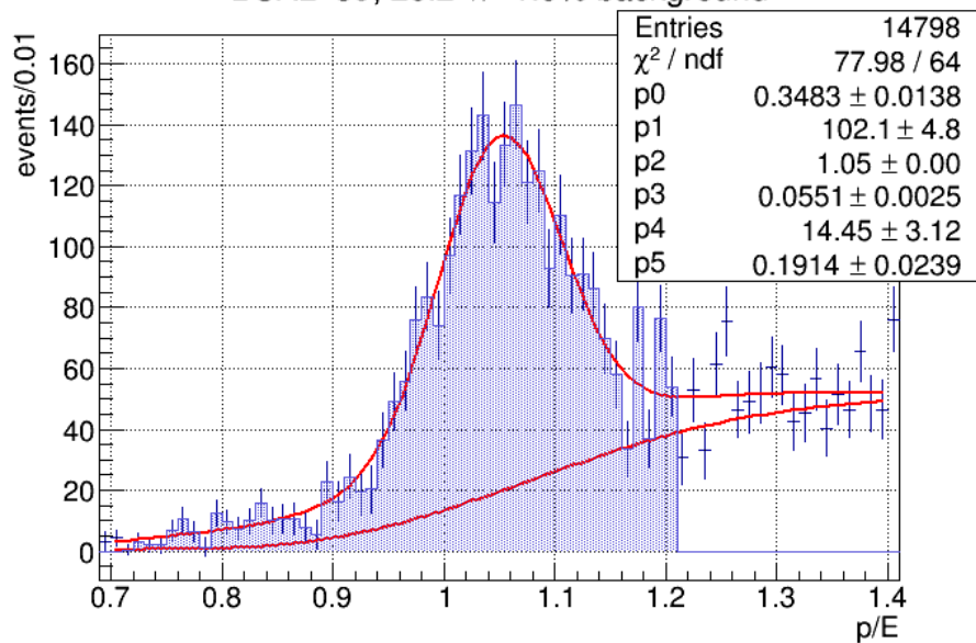
BCAL 3\sigma , 26.2 +/- 1.0% background
