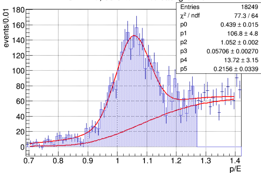
BCAL 4\sigma , 35.5 +/- 1.2% background
