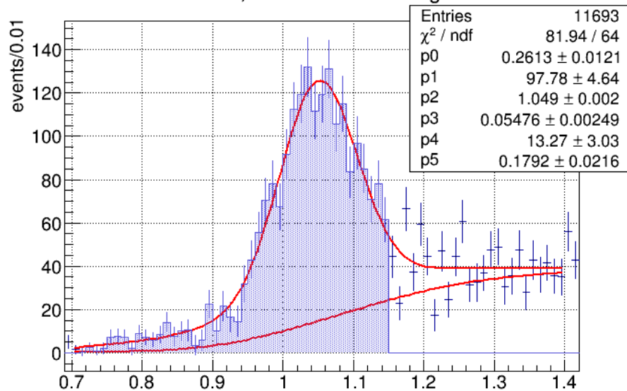
BCAL 4\sigma , 35.5 +/- 1.2% background
