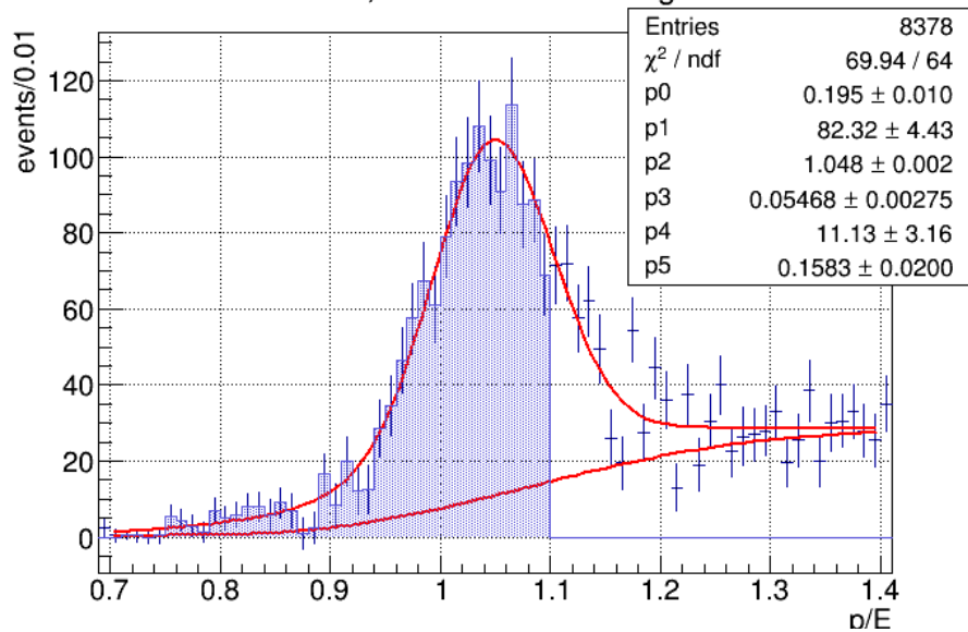
BCAL 3\sigma , 26.2 +/- 1.0% background
