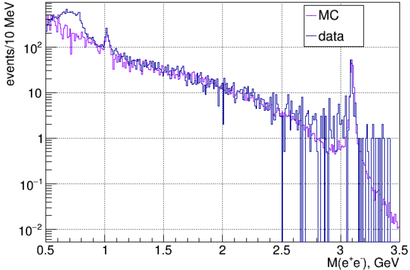
2017(L+H) data vs MC with random hits ( 1\sigma cuts)
