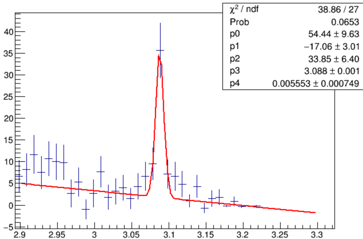
J/ \psi fit of Minv for 8.250000 < E < 8.850000 accidental corrected
