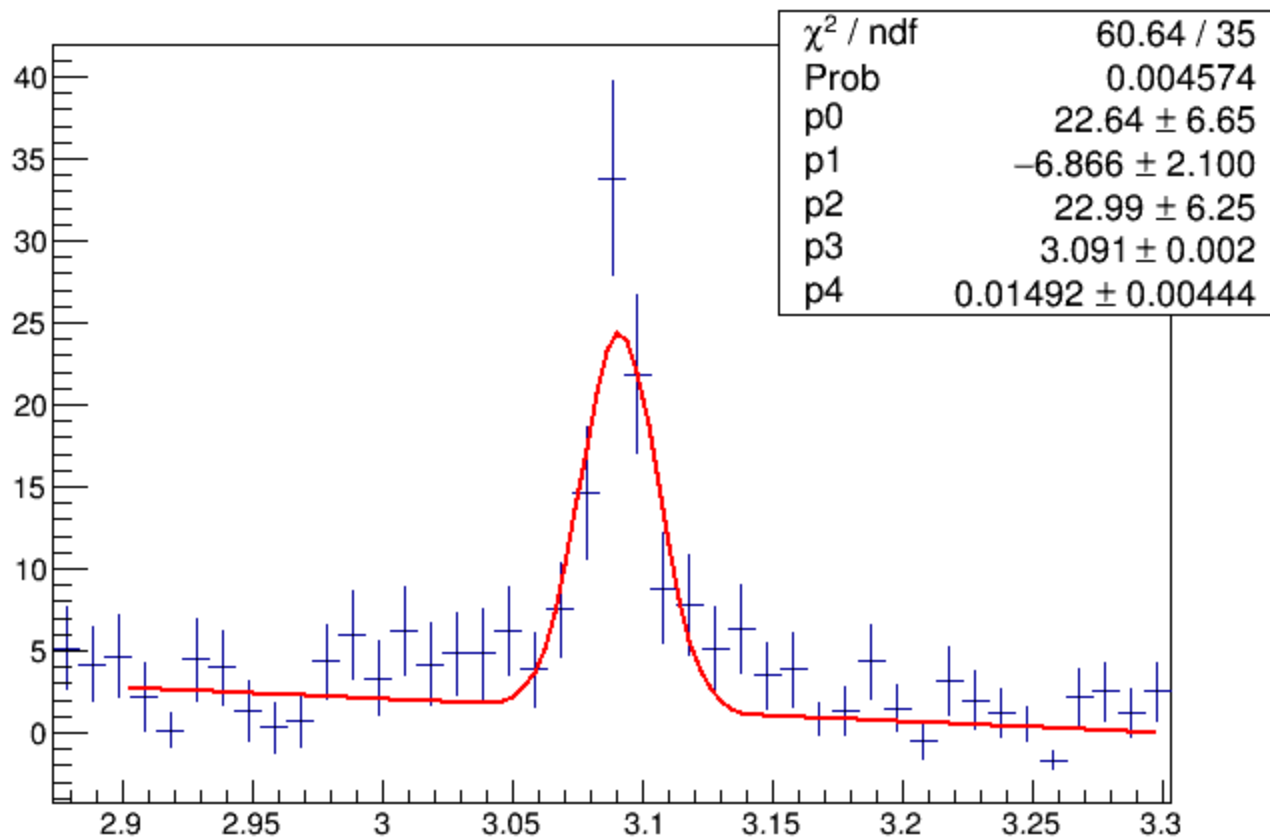
J/ \psi fit of Minv for 10.650001 < E < 11.250001 accidental corrected
