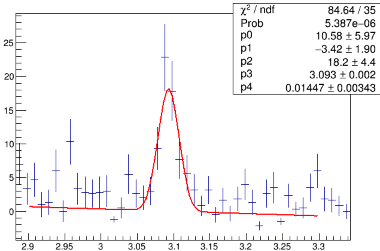
J/ \psi fit of Minv for 10.050000 < E < 10.650001 accidental corrected
