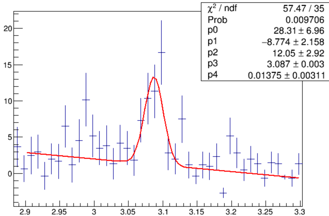
J/ψ fit of Minv for 8.850000 < E < 9.450001 accidental corrected
