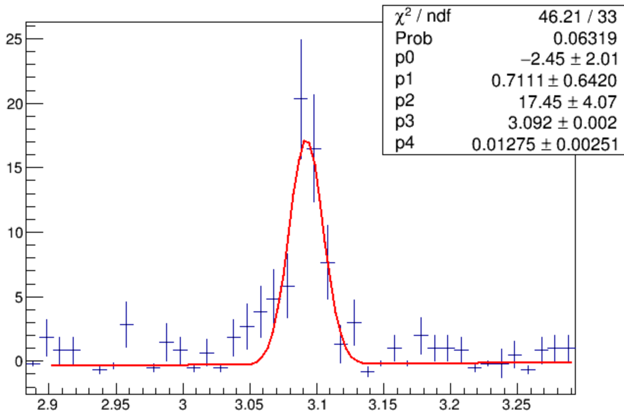
J/ \psi fit of Minv for 11.250000 < E < 11.850000 accidental corrected
