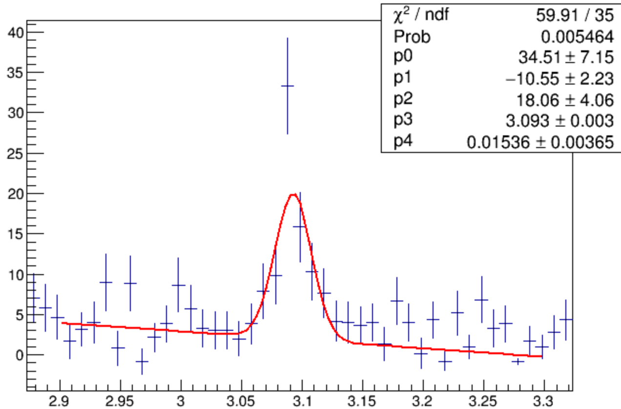
J/ \psi fit of Minv for 9.450000 < E < 10.050000 accidental corrected
