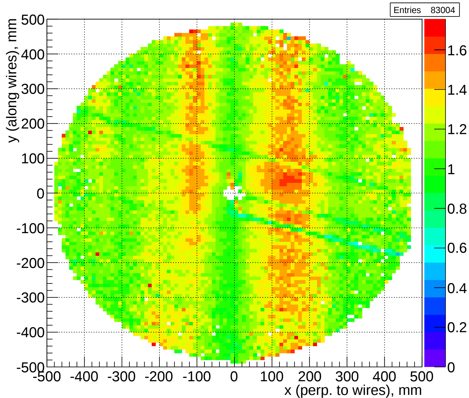
FDC2 Cell5 up/down charge vs x position profile zy projection
