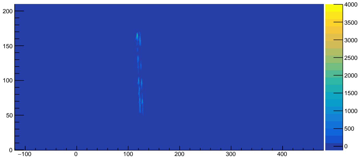
GEM amplitude vs channel and time
