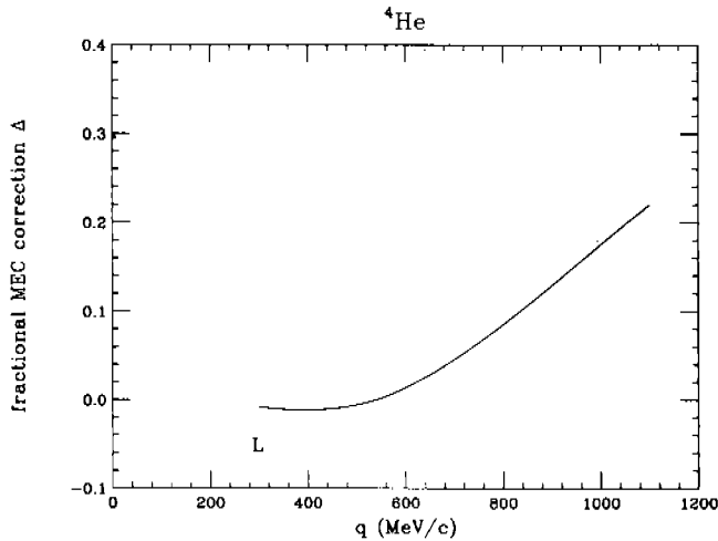
Figure 1: Contribution of MEC to the Coulomb sum.
