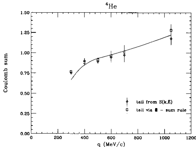
Figure 2: Experimental Coulomb sum compared to theory. The error bars include both the statistical and systematic uncertainties, the calculation includes the contribution of two-body charge operators.
