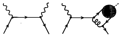
Fig. 5. Lowest-order hard subprocesses for deeply virtual photon and meson production.
