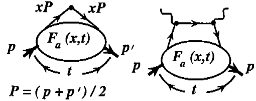
Fig. 3. Form factor and wide-angle Compton scattering amplitude in terms of nonforward parton densities.
