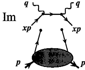
Fig. 2. Lowest order pQCD factorization for DIS.
