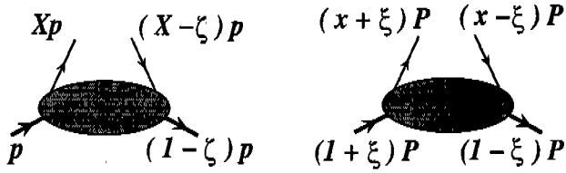
Fig. 6. Comparison of NFPDs and OFPDs.
