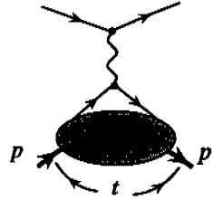
Fig. 1. Elastic eN scattering in one-photon approximation.
