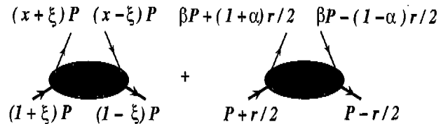
Fig. 7. Comparison of GPD and DD descriptions.
