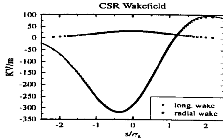
Figure 2: CSR wakefield on the bunch at steady state; the dots are the simulated wakefields with the rms of the macroparticle centroid distribution being \sigma_s , and the solid curve is the analytical longitudinal wakefield for the effective bunch length \sigma_s^{\text{eff}} . Here \sigma_m/\sigma_s = 0.4 .
