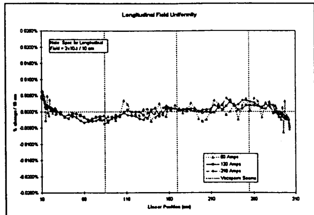
Figure 5: Longitudinal Field Uniformity DY001
