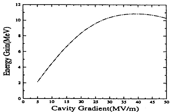
Figure 4: Maximum energy gain by a 350 keV electron beam traversing a 5-cell CEBAF cavity.
