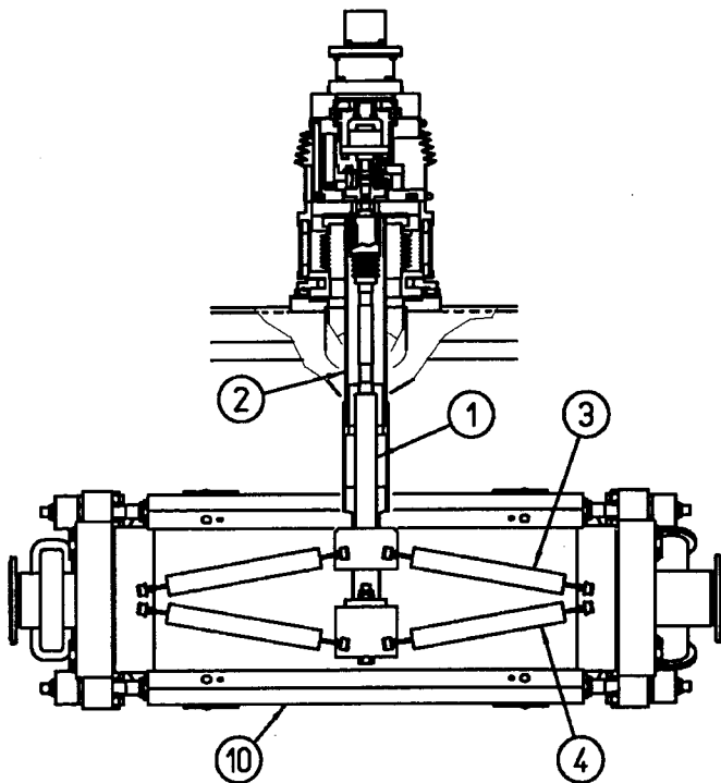
Fig. 2: Scissors Type Jack
