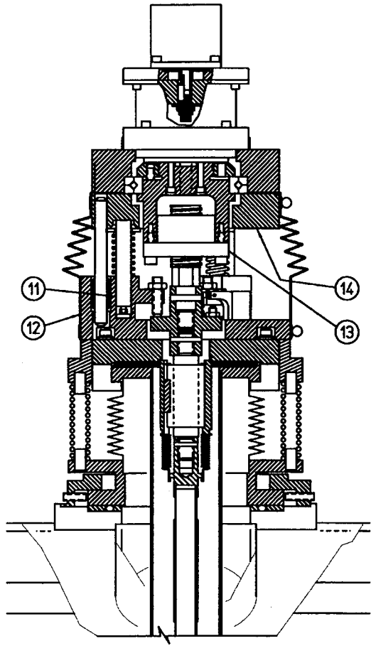
Fig. 4: Drive Assembly
