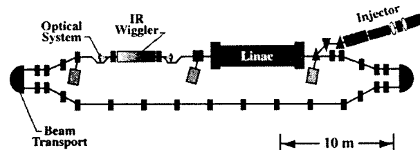
Figure 6. Schematic layout of the JLab IR FEL.
