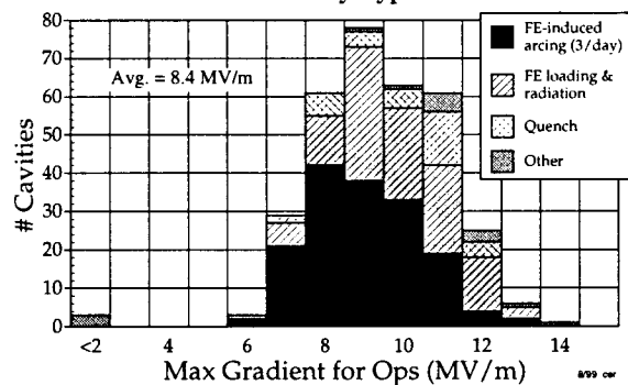
Figure 2. Gradient limitations for CEBAF cavities.
