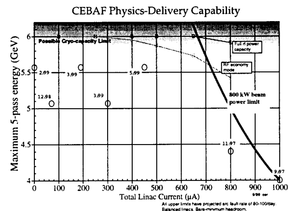
Figure 4. Approaching the limits of CEBAF.
