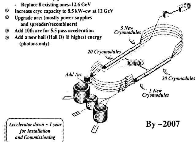
Figure 5. CEBAF upgrade to 12 GeV.
