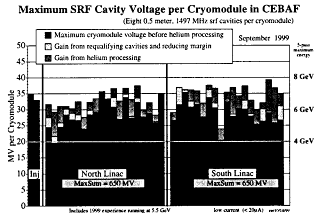
Figure 3. Peak capability of the CEBAF cryomodules.
