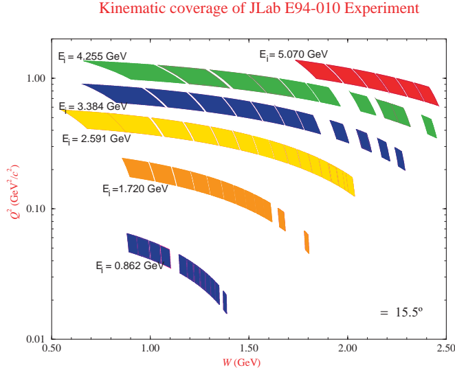
Figure 1. E94-010 Kinematics
