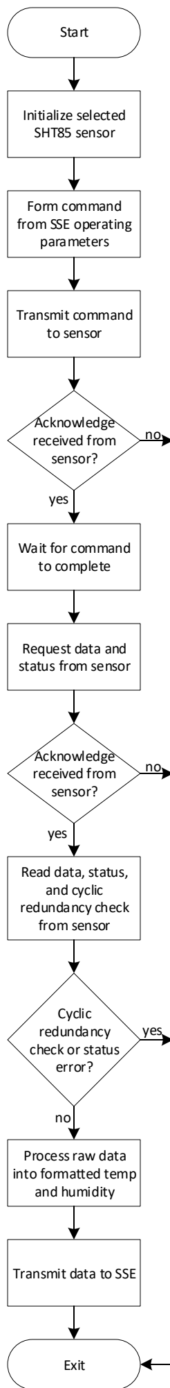
Single Shot Data Acquisition Mode Flowchart 1/7/2020 M. A. Antonioli
