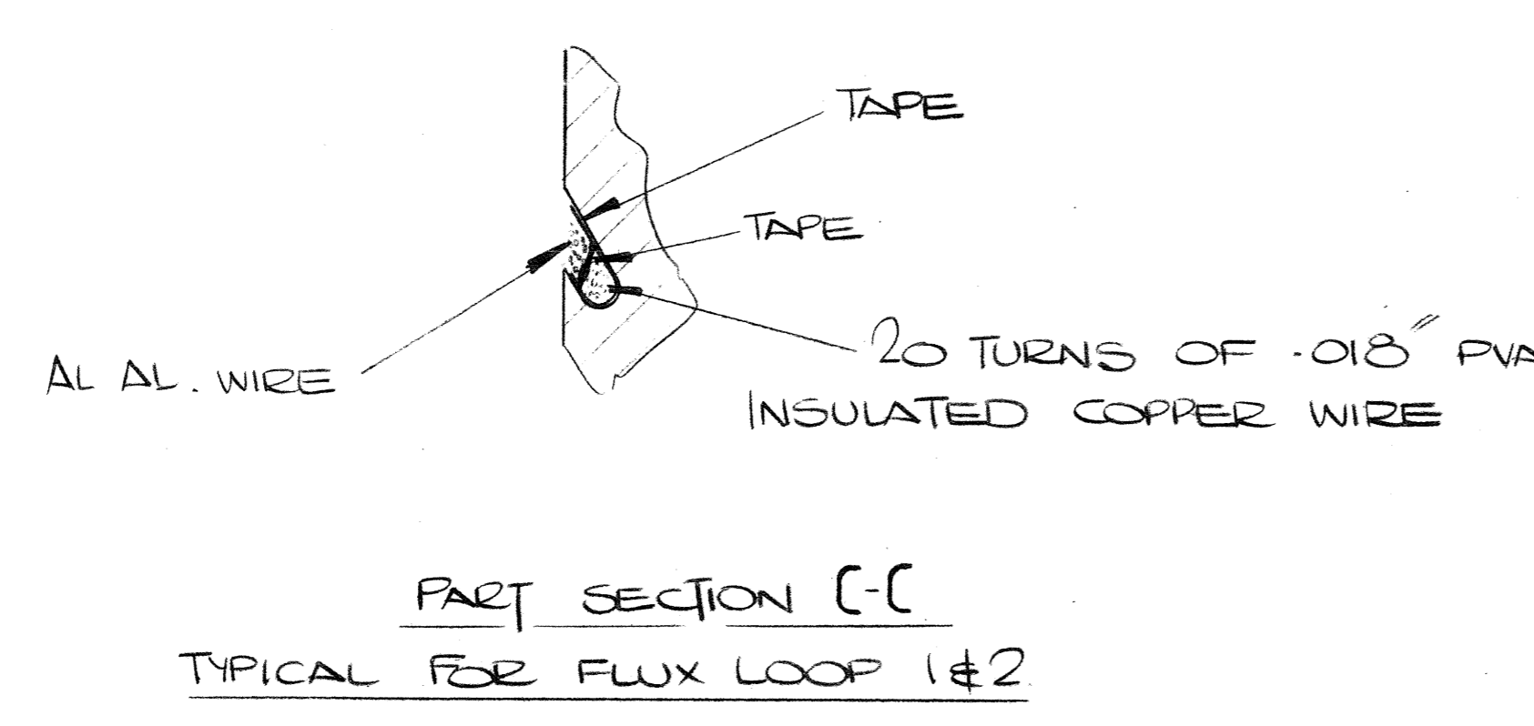
DEVELOPMENT OF COIL SHELL
