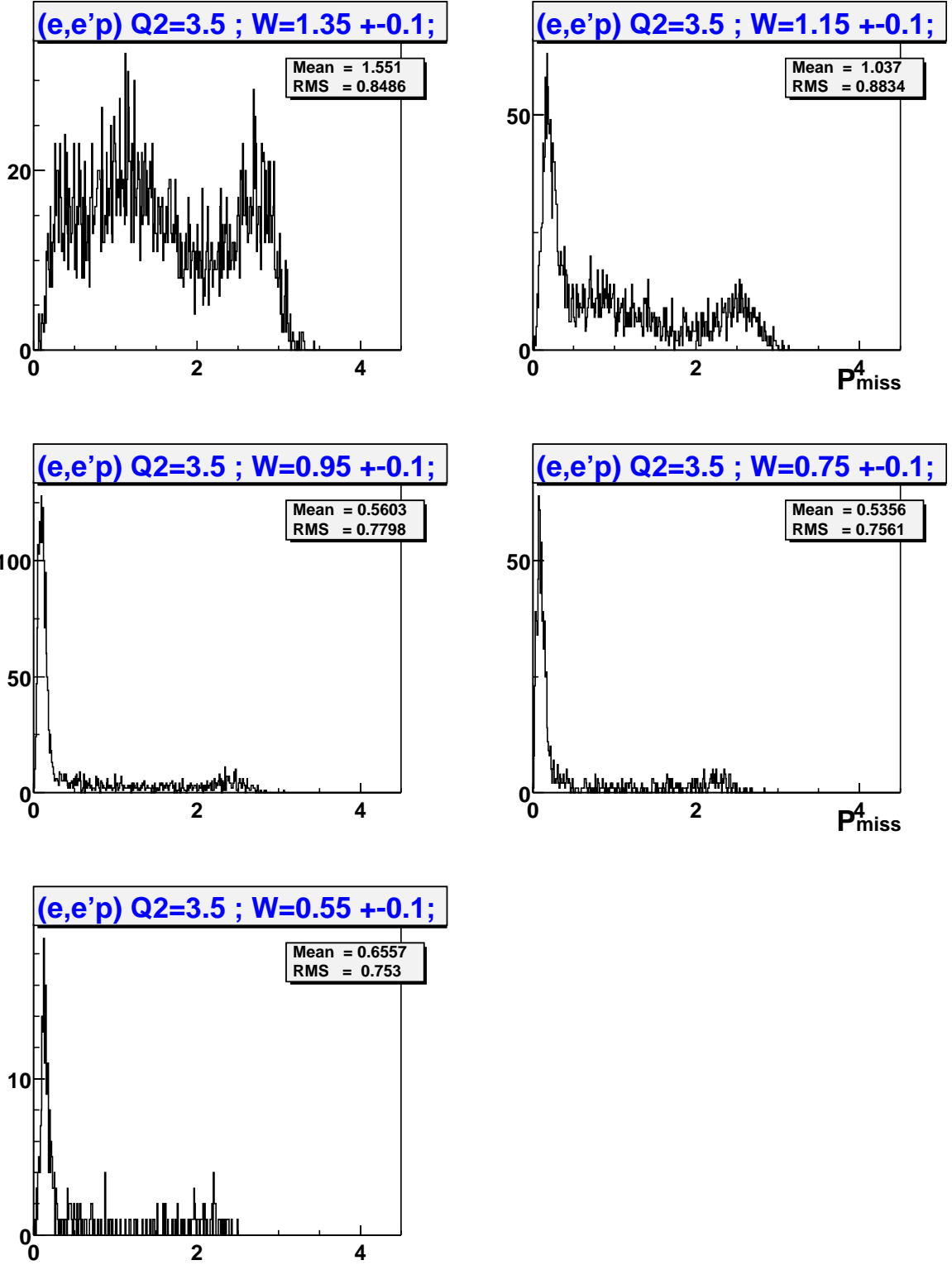
Figure 27: The p_m distributions for {}^3\vec{H}e(e,e'p) at Q^2 of 2.5 (GeV/c) ^2 and 3.5 (GeV/c) ^2 for five W values. The scales are in GeV/c.
