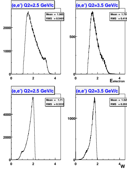
Figure 25: The inclusive electron spectra for the reaction {}^3\bar{H}e(e, e') at an incident energy of 4.4 GeV for two values of Q^2 . The lower graphs are the invariant mass distributions. The scales are in GeV.
