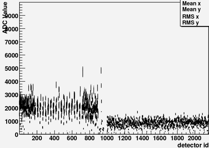
LMS ADC Value versus Channel Id for Run 05153
