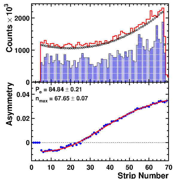
FIG. 6: (top) Typical Monte Carlo simulated Compton spectra for a single detector plane; ideal (black open circles), with noise (red) and with detector efficiency (blue, shaded). (bottom) The Compton asymmetry extracted from the simulated spectrum including detector efficiency (blue circles), and a two parameter fit to the calculated asymmetry (red line). The input asymmetry was 85%.
