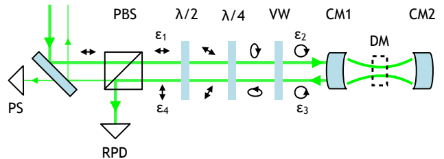
FIG. 4: Scheme for maximizing the circular polarization at the cavity. Laser light entering the system passes through a polarizing beam splitter (PBS), half-wave plate ( \lambda/2 ), quarter-wave plate ( \lambda/4 ), and vacuum window (VW) before it is either reflected off the cavity entrance mirror (CM1) or becomes resonant in the cavity. Note that in this figure, the element VW also includes 3 steering mirrors, which are incorporated in the model but left out of the figure for simplicity. Depending on the polarization state at CM1, reflected light will either arrive in reflected photo-diode (RPD), used for frequency-locking feedback, or be sampled by the polarization signal (PS) photodiode behind a steering mirror. Light arriving at the cavity entrance mirror is fully circular when there is no signal in PS. Before the experiment, with part of the beamline vacuum pipe removed, it was possible to do a direct measurement (DM) of the circular polarization in the cavity.
