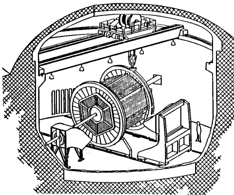
Figure 4: LAS/Hall B 100' Diam.
