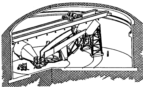
Figure 6: Hall C 150' Diam.
