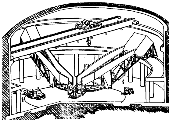
Figure 1: Hall A 185' Diam.
