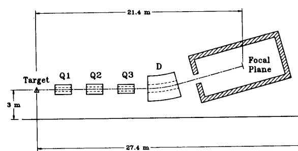
Figure 7: Electron Spectrometer - Hall C
