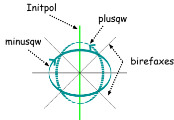
Fig. 2. Polarization ellipse, representing the shape circumscribed by the electric field vector, for each polarization state. An asymmetric phase shift \Delta creates a small residual linear polarization of opposite sign for the two helicity states.
