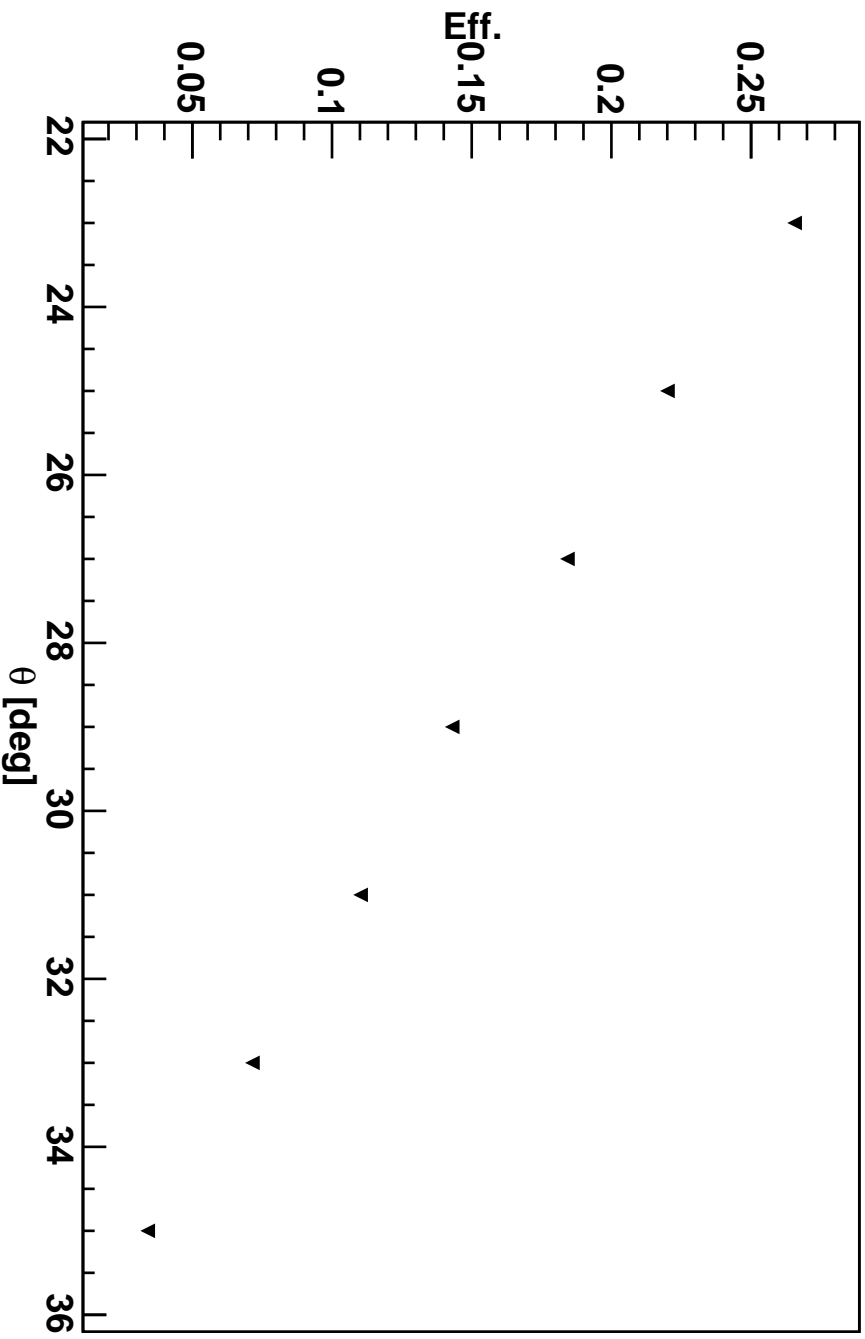
CDF, my baffles Track Propagation Efficiency, e - , DIS, 22.0° < θ < 35.0°, x>0.2
