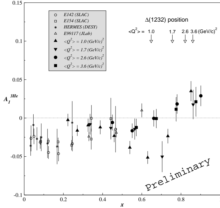
Fig. 2. Preliminary result of A_1^{3\text{He}} . The error bars are statistical only.
