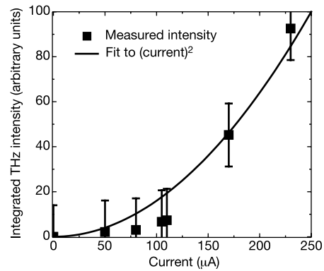
Figure 4 Measured THz intensity as a function of beam current (square symbols), showing the quadratic dependence expected for coherent emission (solid line). We note that in our experiments we were able to observe considerable changes in spectral weight depending on operating conditions, and we were able to enhance certain spectral regions in a controlled way via the machine parameters. Thus the electron bunch distributions were not purely gaussian. This accounts for the large error bars.
