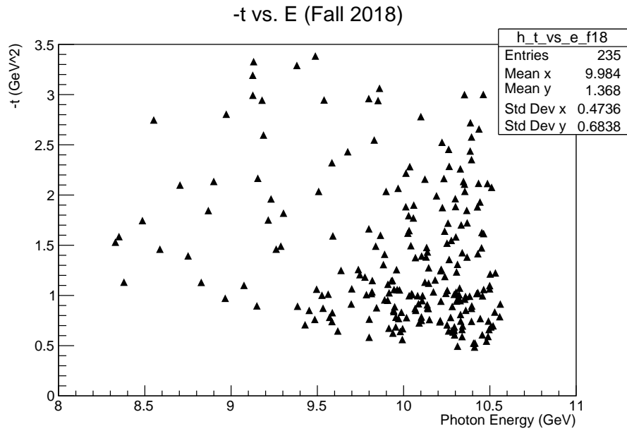
FIG. 92. 2D distribution of the momentum transfer and the photon energies for the Fall 2018 dataset.
