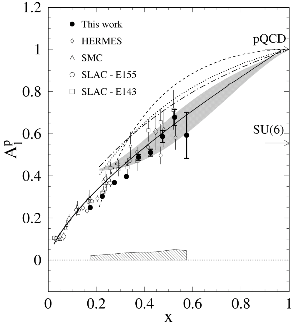
Figure 4: Results from the Jefferson Lab spin experiment with CLAS: The asymmetry A_1 indicates the fraction of the proton spin carried by the quarks. The more of the energy of the proton is carried by a single quark (right side of the graph), the more likely it is aligned with the proton spin. The results agree best with the “Hyperfine perturbed Quark Model” by Nathan Isgur (grey band) which takes “color magnetism” into account. On the opposite end of the graph, we find that the average spin of quarks carrying only a small fraction of the nucleon energy nearly cancels out to zero. This is due to a large “sea” of quark-antiquark pairs that pop in and out of existence inside the nucleon, with their spins preferably aligned opposite to the overall nucleon spin.
