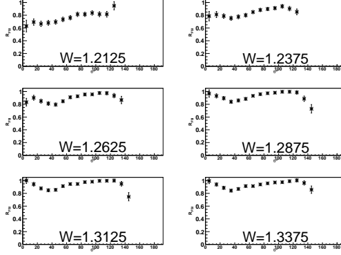
Figure 2. The FSI correction factor R_{FSI} as a function of (\theta_{\pi}^*) is represented by the stars for different W bins at Q^2 = 0.7 \text{ GeV} .
