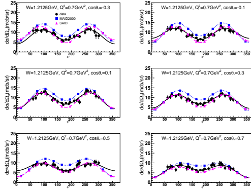
Figure 3. (Color online) A typical example of the \phi_{\pi}^* -dependent cross section for different \cos\theta_{\pi}^* values at Q^2 = 0.7 \text{ GeV} and W = 1.212 \text{ GeV} in comparison to MAID2000 (blue dotted line) and SAID (purple dashed line) predictions. Black solid line is the fit to extract structure functions.
