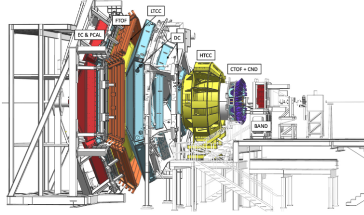
Figure 1. A diagram of the CLAS12 detector highlighting relevant subsystems of the forward and central detectors. Three of the forward detector’s six sectors are visible. Taken from [1].
