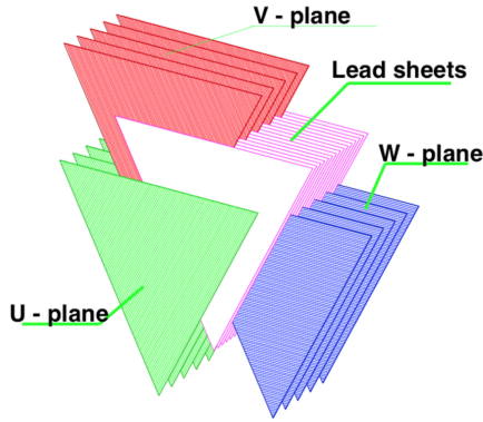
Figure 4. Schematic representation of the calorimeters' three views taken from [9].
