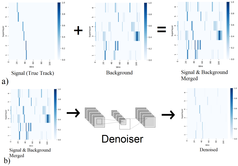
Figure 6. a) The top row demonstrates the process of adding spurious noise to a clean track to synthetically create raw hits as measured by the DC. b) The bottom row demonstrates how the de-noiser can be applied to the raw hits to return cleaner denoised data. Taken from [3].
