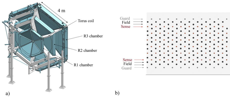
Figure 3. a) Diagram showing the three regions (R1, R2, R3) of the DC, each region containing two superlayers. The forward detector's six sectors are also visible. b) Schematic of the wire layout for one superlayer, with each superlayer containing 6 layers of sense wires (red). The view is a cut perpendicular to the wire direction. Both images are taken from [7].
