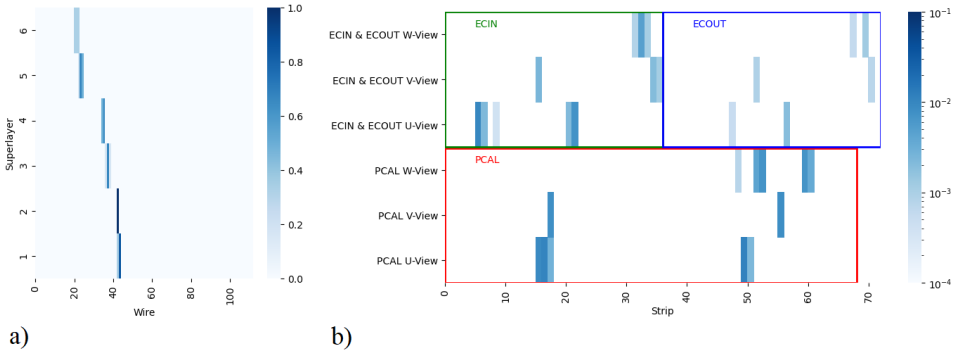
Figure 5. a) An example of a DC image containing an electron track in a given sector. The colour axis represents the number of layers with the same wire number, divided by six for normalisation. b) An example of an ECAL image containing all ECAL hits in a given sector for a single event. The colour axis represents the energy deposited in each strip divided by three. Taken from [3].
