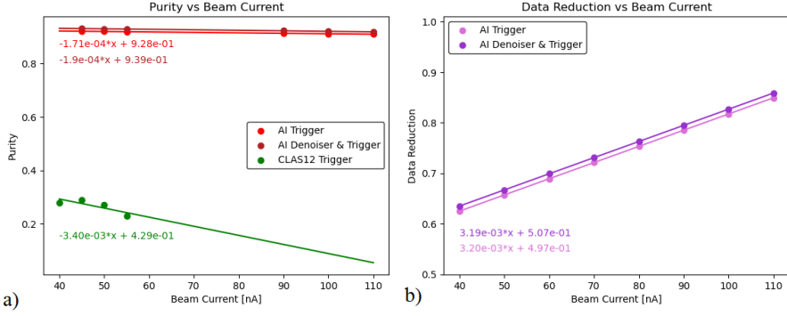
Figure 8. a) The purity of the AI (red) and conventional CLAS12 (green) triggers as a function of beam current. b) The data reduction achieved by the AI trigger relative to the CLAS12 trigger. The purity and data reduction is shown for the AI trigger with and without the denoiser. For both AI triggers the cut on the response was placed at 0.08 in both plots. Both plots taken from [3].
