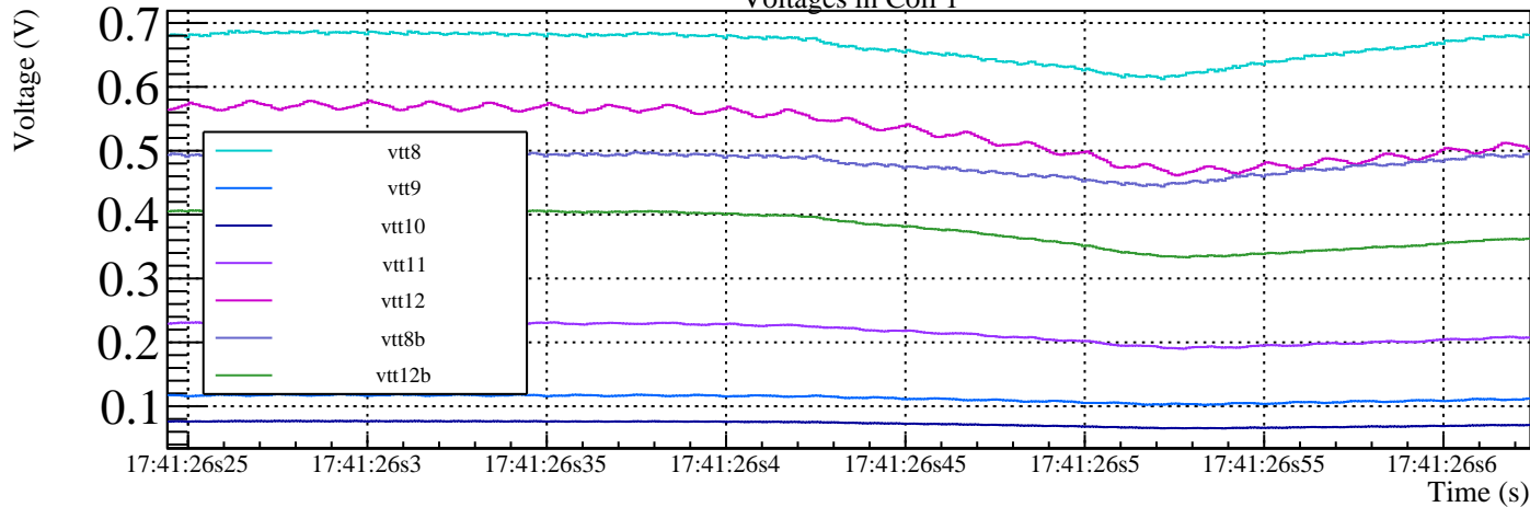
Voltages in Coil 1
