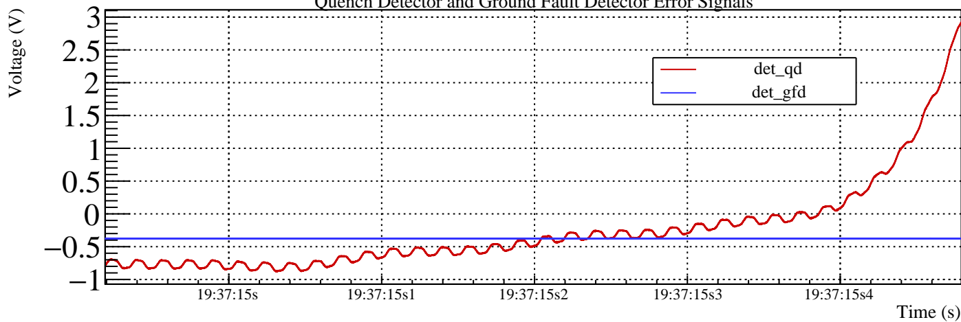
Voltages across Leads
