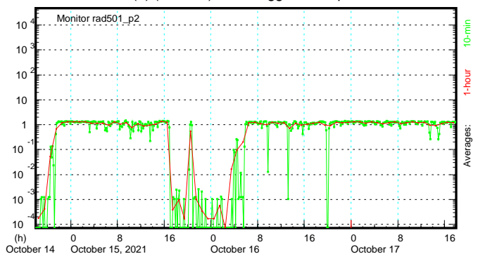
RM-501(n) (mrem/h) - XD Tagger Transport Tunnel
