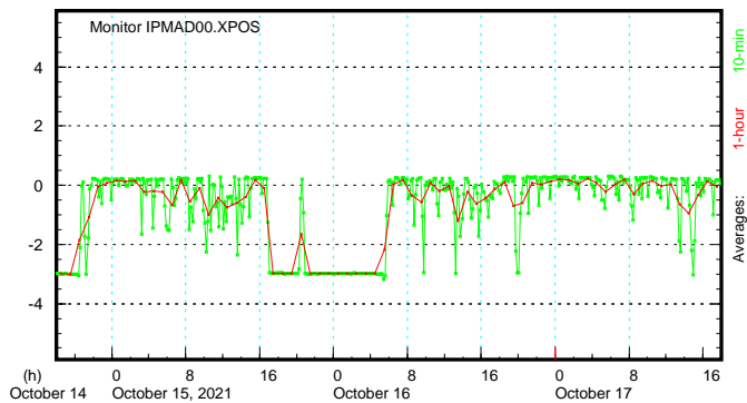
X Beam Position at IPMAD00
