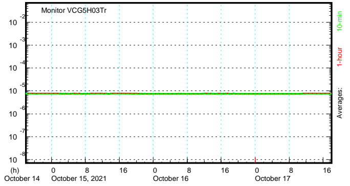
XD Vacuum at the Photon Line in XD (Torr)
