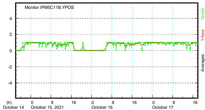
Y Beam Position at IPM5C11B
