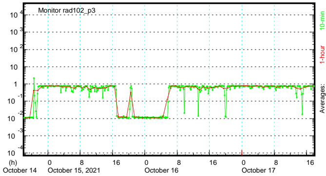
RM-102( \gamma ) (mrem/h) - XD Tagger Beam Line
