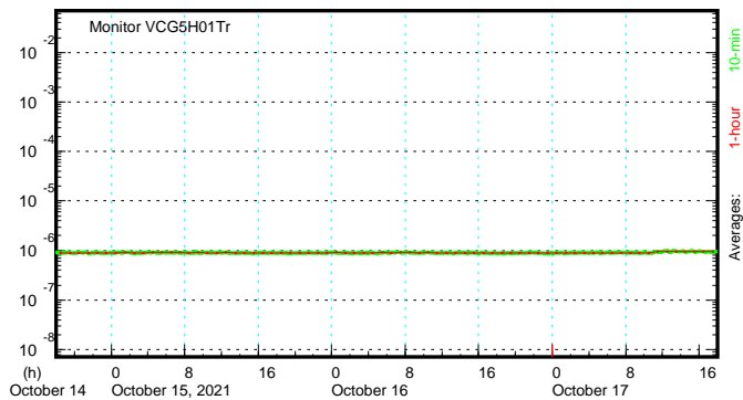
XD Vacuum at gamma pipe (Torr)
