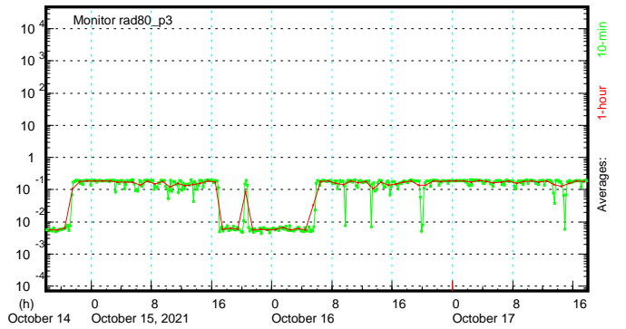
RM-80( \gamma ) (mrad/h) - Upstream of Solenoid magnet (BL)
