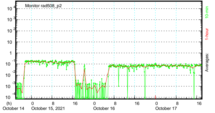
RM-508(n) (mrem/h) - XD Downstream Solenoid
