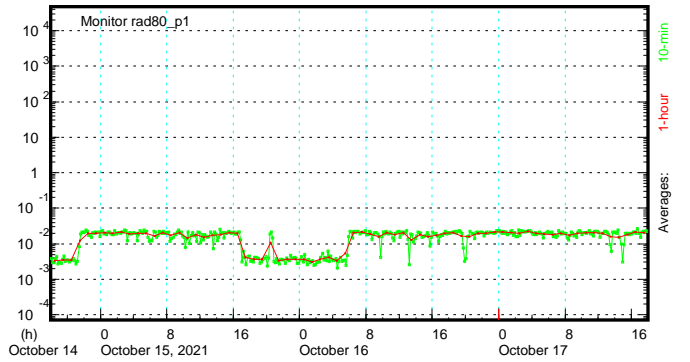
RM-80( \gamma ) (mrad/h) - Downstream Cave Wall (BL)
