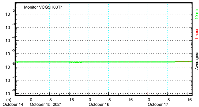
XD Vacuum beyond Tagger Magnet (Torr)
