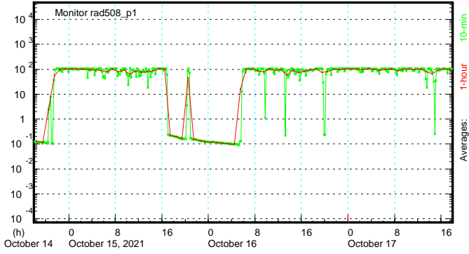
RM-508( \gamma ) (mrad/h) - XD Collimator Cave
