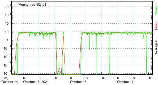
RM-102(n) (mrad/h) - XD Tagger Electr. Racks
