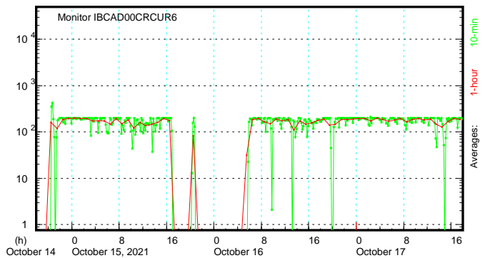
Hall D: Beam Current (nA)
